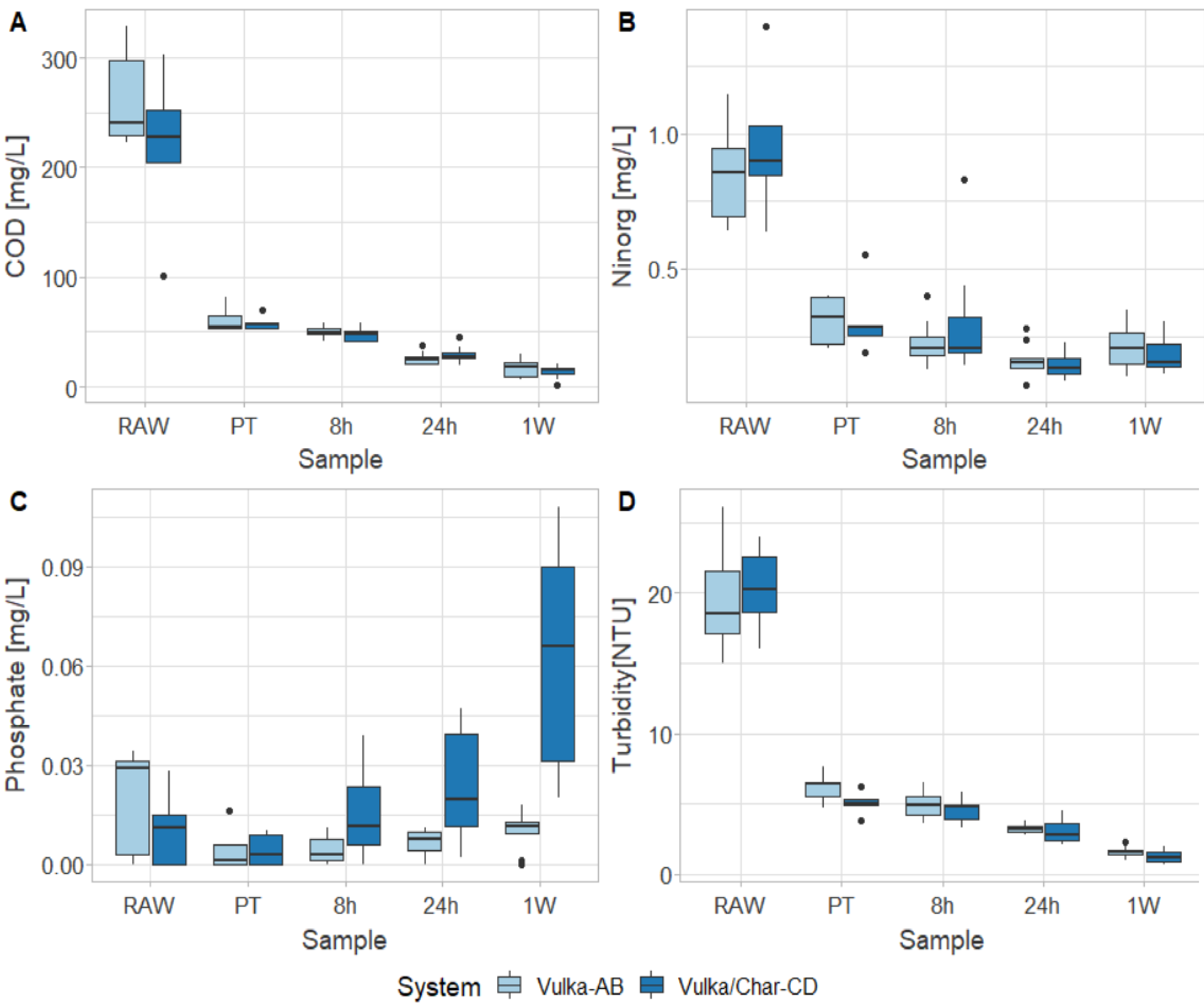
Figure 2: Average COD, N=5 (A); Ninorg, N=5 (B); \text{PO}_4\text{-P} , N=5 (C) and turbidity, N=5 (D) measured in two different systems (Vulka-AB and Vulka/Char-CD). Measured in raw greywater (RAW), pre-treated greywater (PT), after 8h, 24h and 1 week (1W) of recirculation in the green wall.
