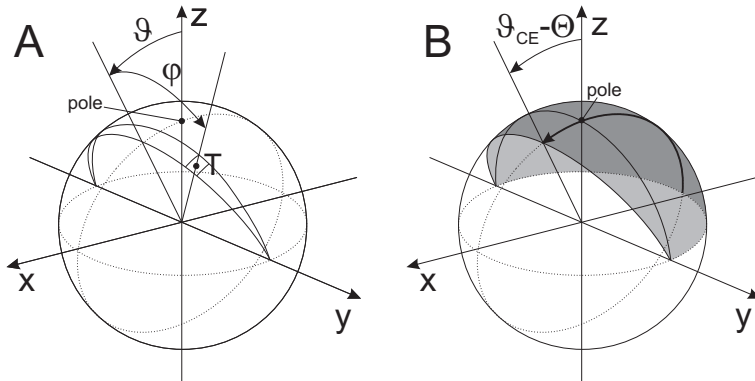
Fig. 2. Schematic presentation of the articular sphere and the coordinate system.
