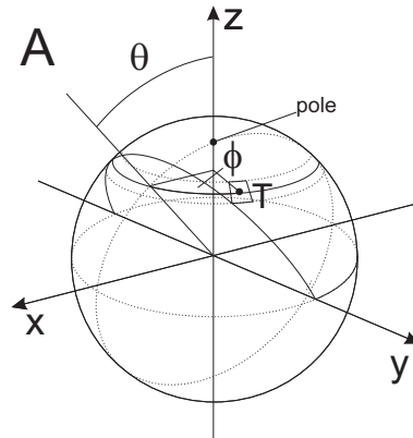
Fig. 3. Schematic presentation of the articular sphere in the spherical coordinate system.
